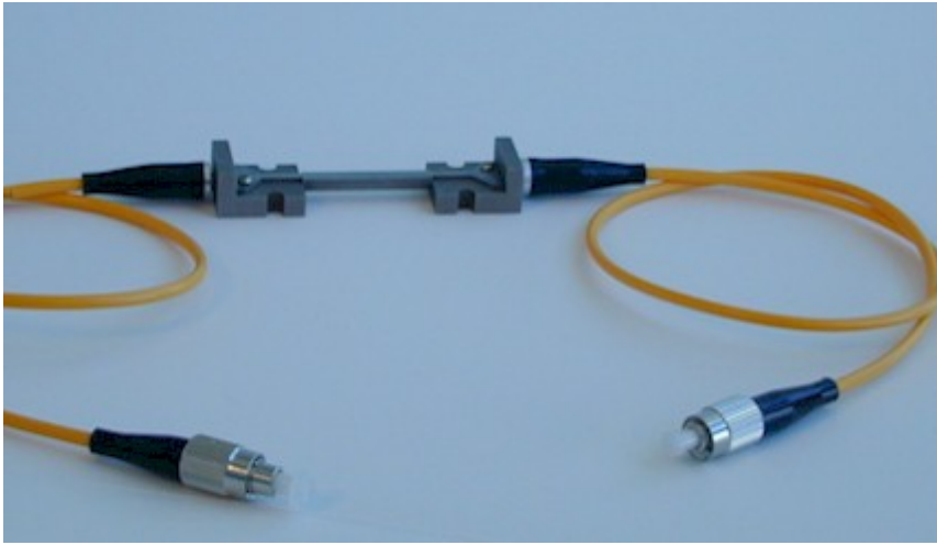
Fiber Bragg Grating Strain Sensor for Surface Mount
