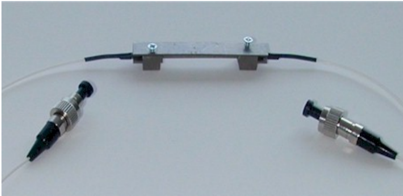
FBG Strain Sensor with high profile surface mount
