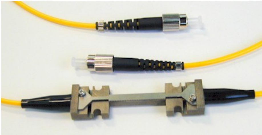
Temperature Compensated Fiber Bragg Grating Strain Sensor
