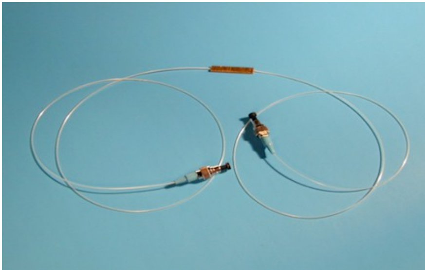
FBG Strain Sensor with small form surface mount
